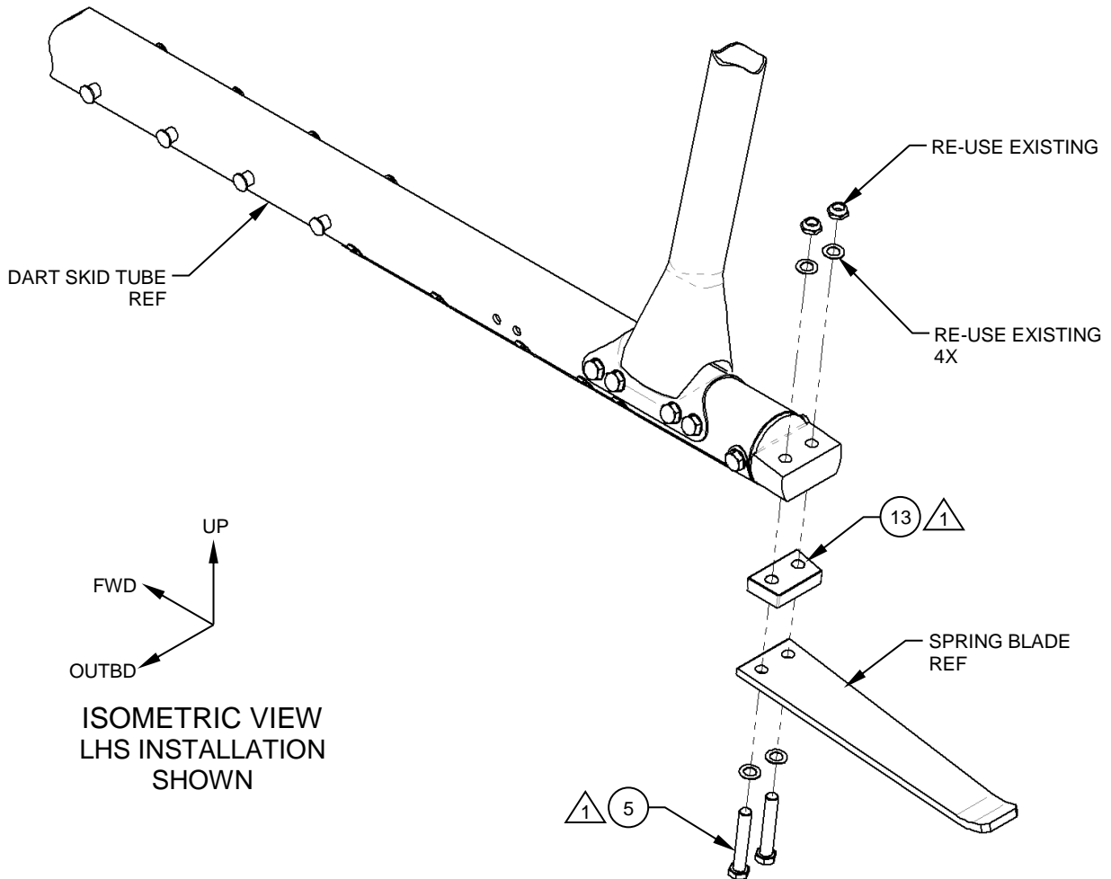
Figure 6 Spacer, Detail (Item 13) Dart Installation shown
