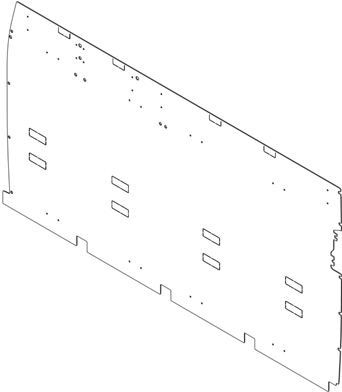
AFT LHS Sliding Door Floor Protection, Assy Shown Item 23
