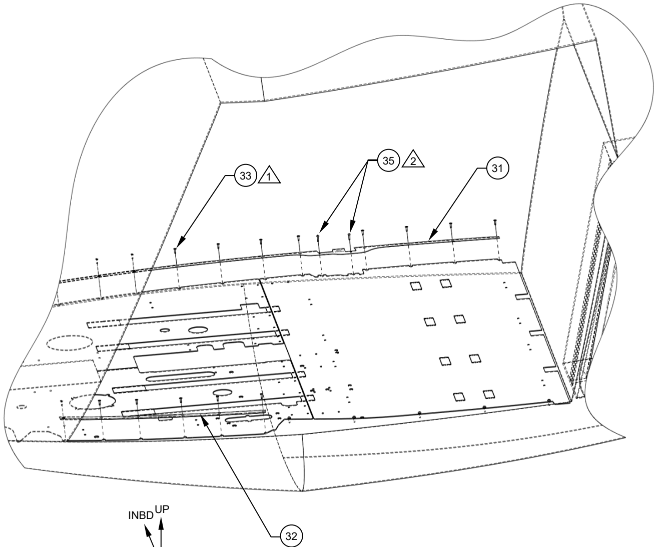
Figure 5 Some Items Removed for Clarity
