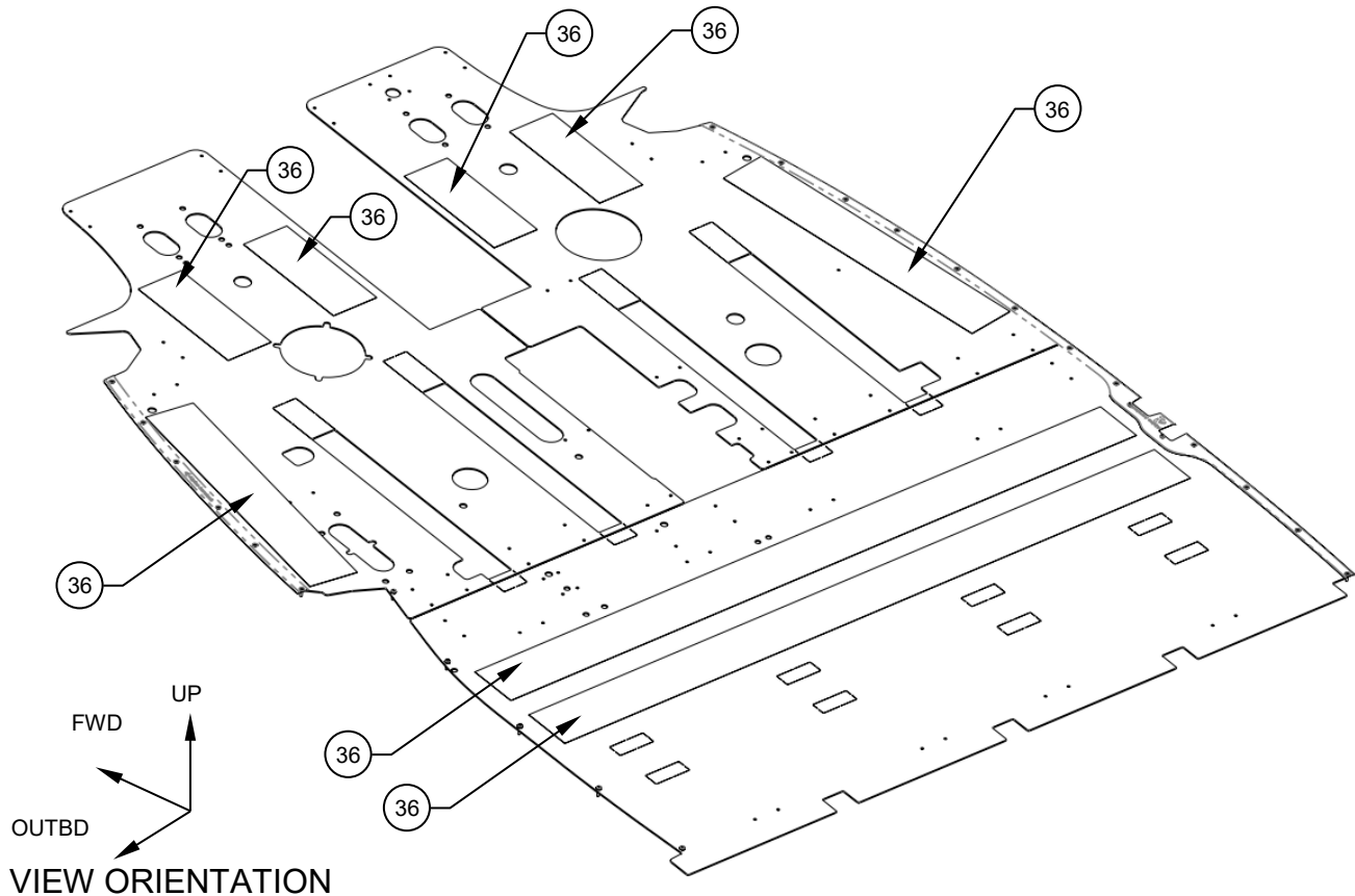
Figure 7 Suggested Grip Tape (Item 36) Installation Shown Some Items Removed for Clarity
