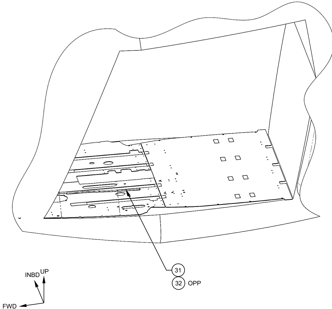
Figure 5 LHS Shown RHS Opposite Some Items Removed for Clarity
