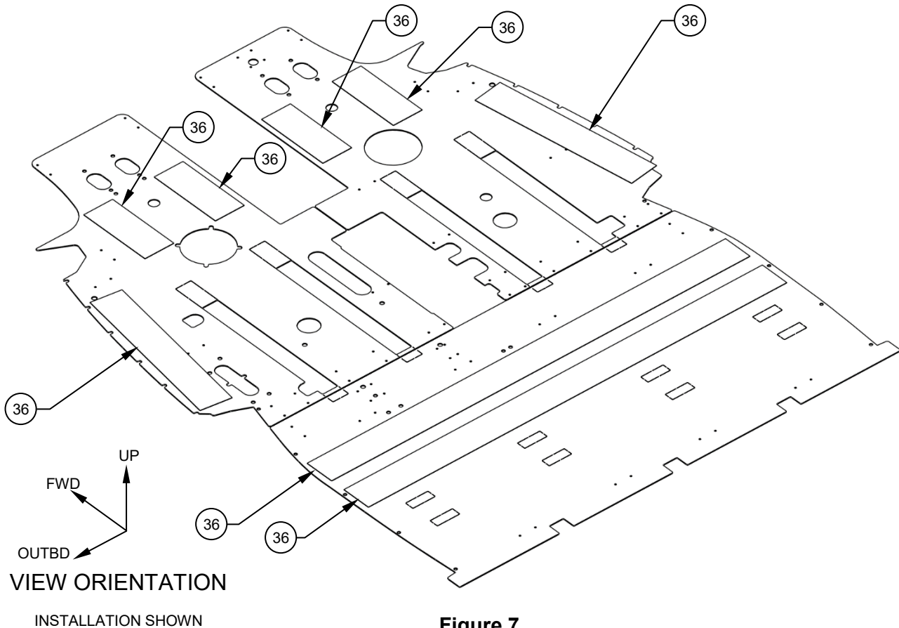
Figure 7 Suggested Grip Tape (Item 36) Installation Shown Some Items Removed for Clarity
