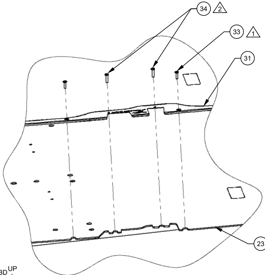
Figure 6 LHS Shown RHS Opposite Some Items Removed for Clarity
