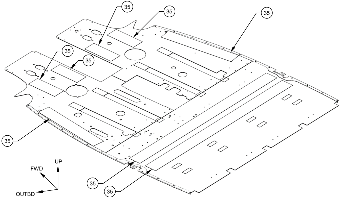
Figure 7 Suggested Grip Tape (Item 35) Installation Shown Some Items Removed for Clarity
