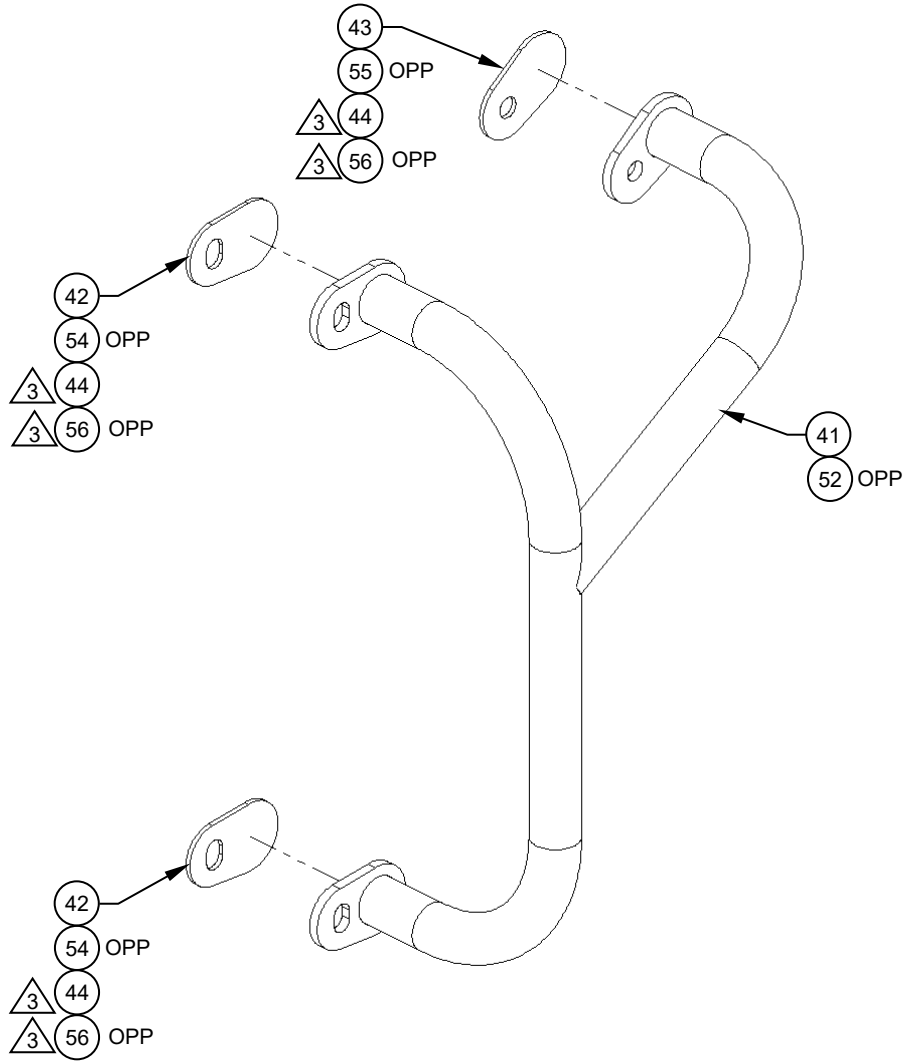
Handle, Assy, LHS AFT (Item 40) Shown Handle, Assy, RHS AFT (Item 52) Opposite
