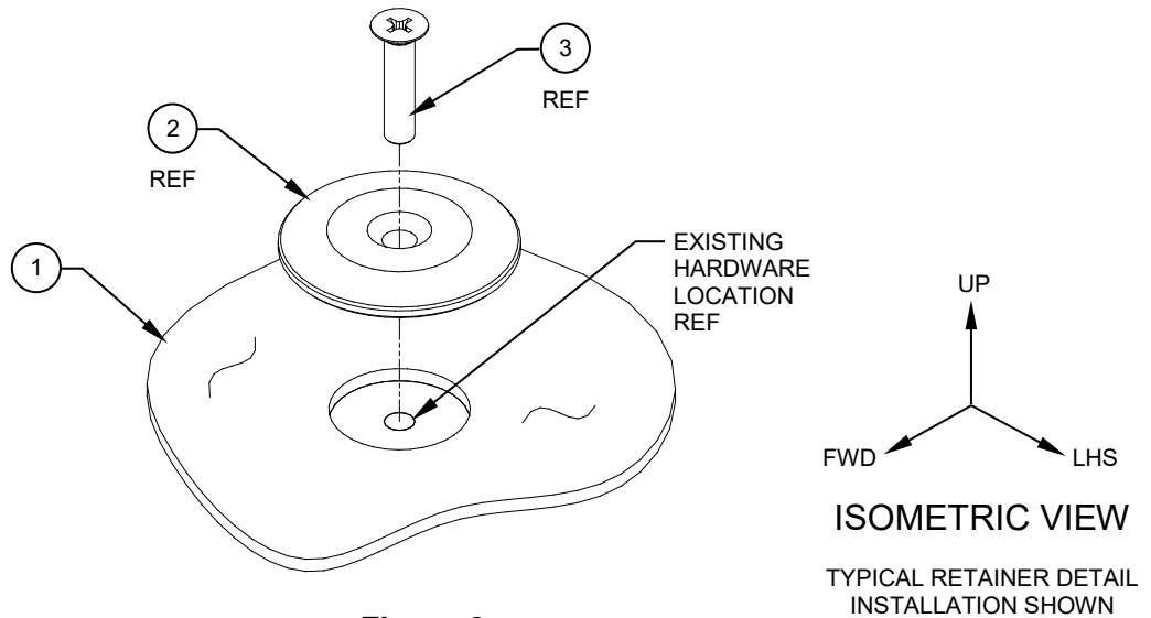
Figure 3 Typical Arrangement
