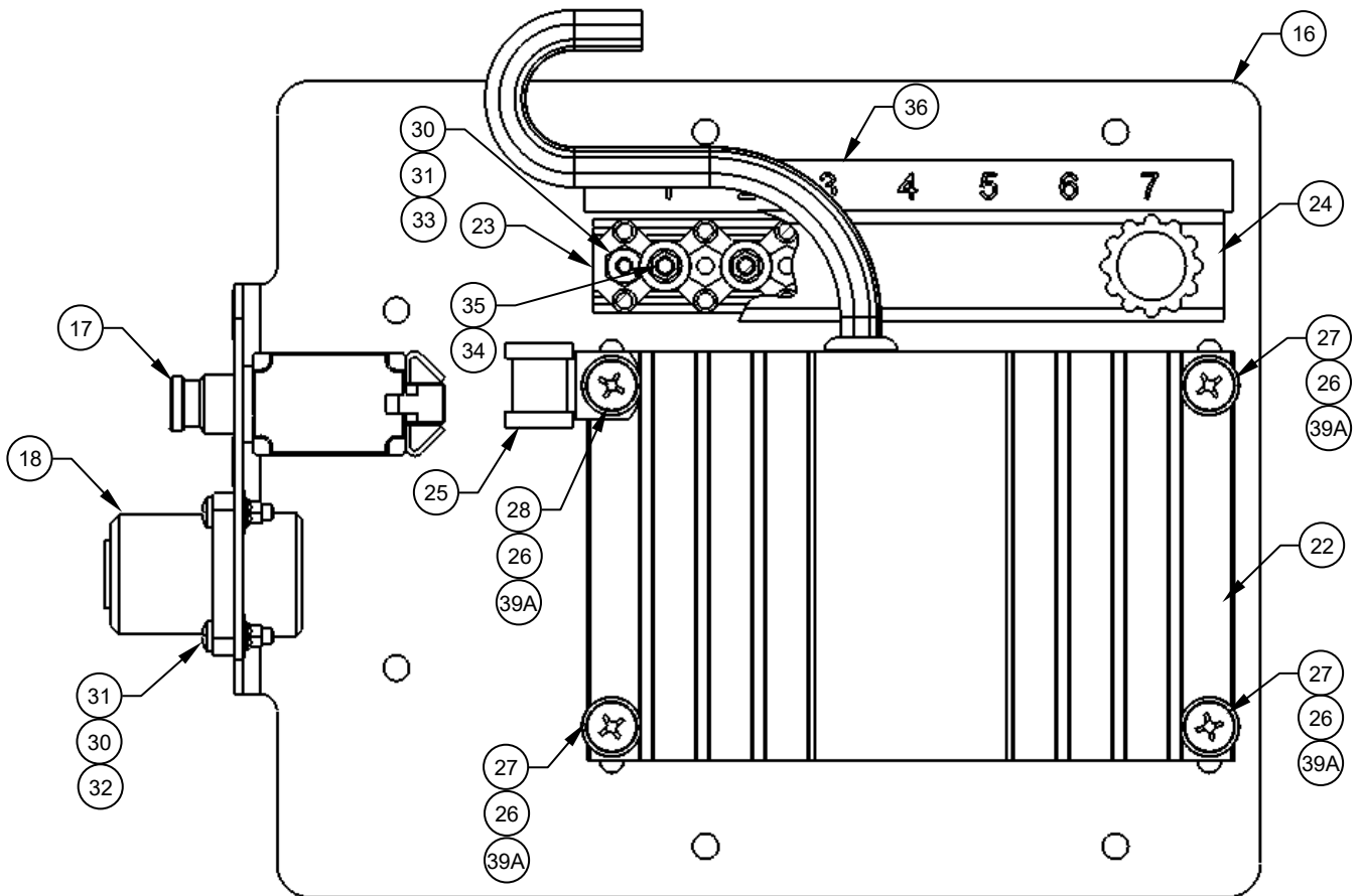
Control Unit, Assy Item 15 Some items not shown for clarity
